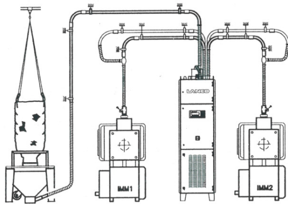
LTX dryer feeding two replication machines from a BIG BAG discharge station with air inlet filter.
