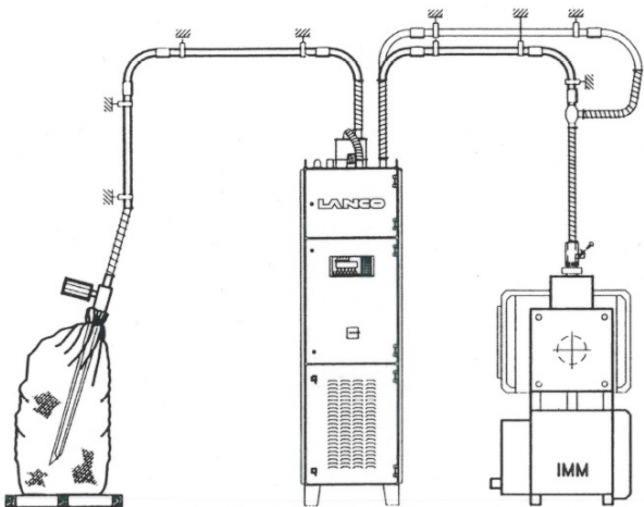
Basic installation of an LTX dryer serving one molding machine directly from a BIG BAG.
